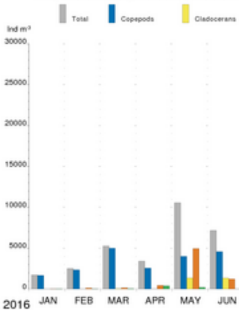
Long Term Ecological Research (LTER) Study Monthly abundance of mesozooplankton collected by WP-2 vertical haul
